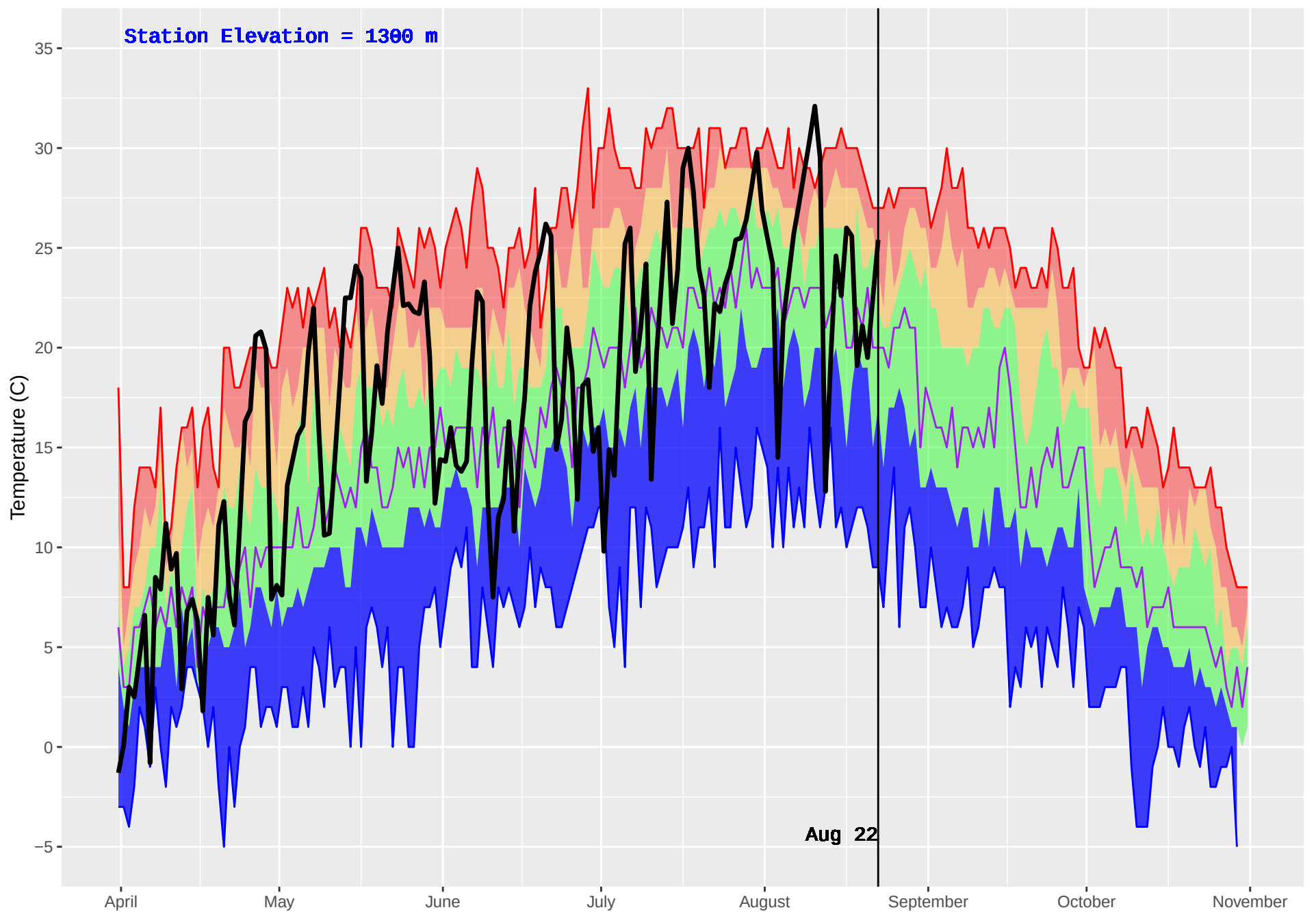
MARION (367) : Historical (1994–2016) and Current (2018) Daily Temperature
