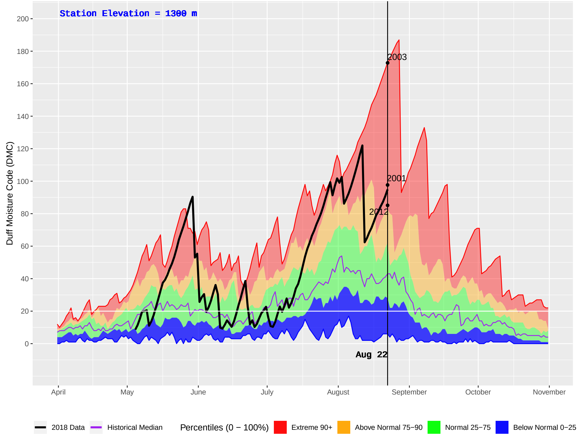
MARION (367) : Historical (1994–2016) and Current (2018) Daily Duff Moisture Code (DMC)
