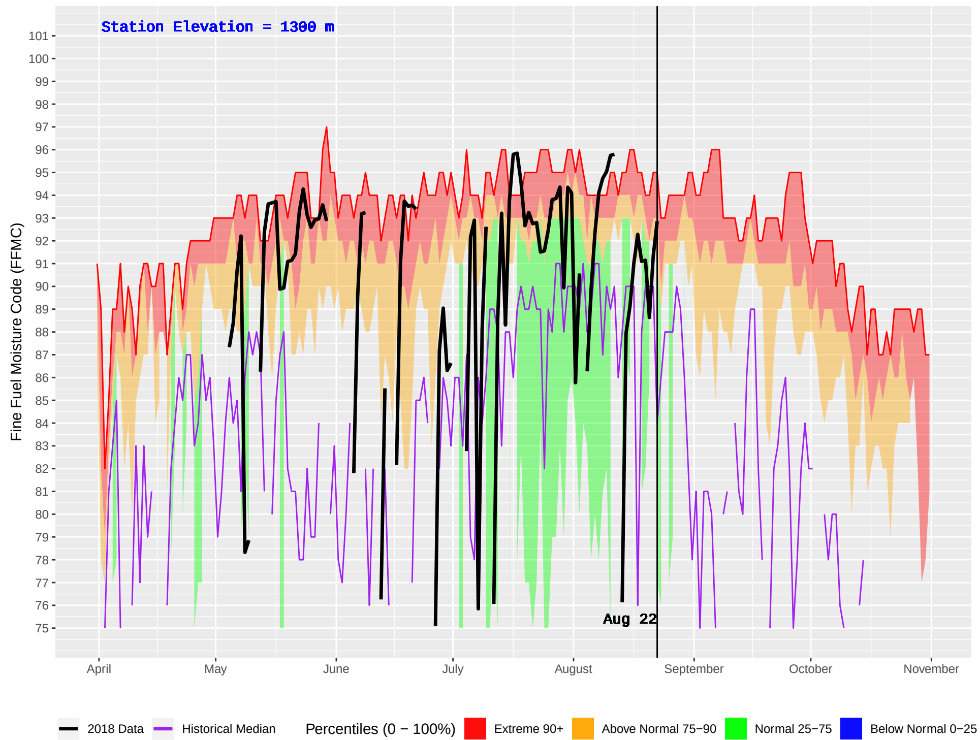
MARION (367) : Historical (1994–2016) and Current (2018) Daily Fine Fuel Moisture Code (FFMC)
