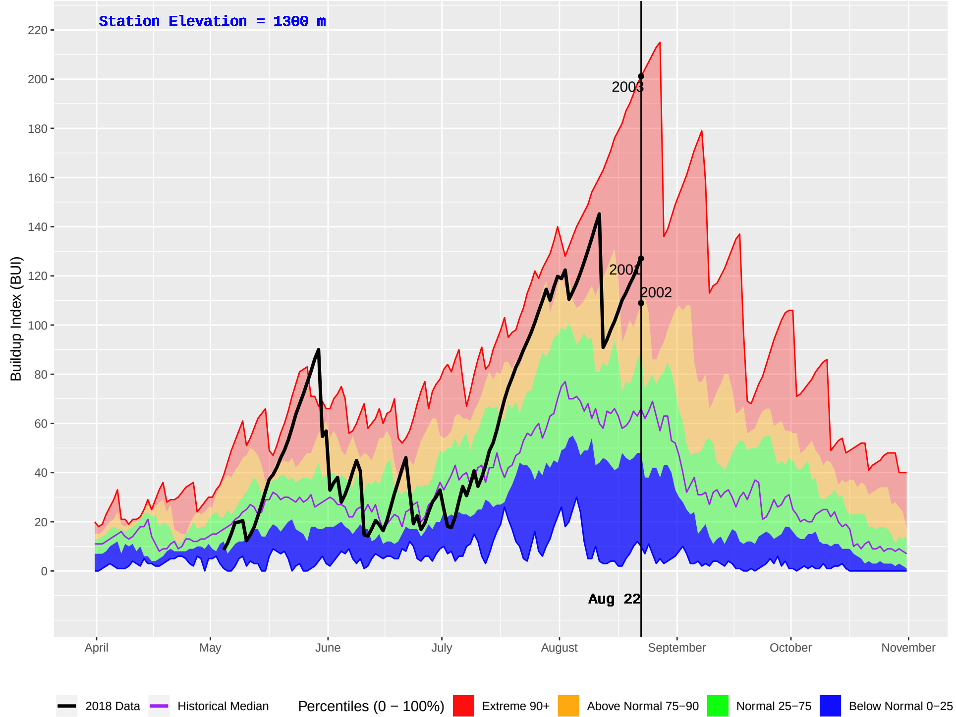
MARION (367) : Historical (1994–2016) and Current (2018) Daily Buildup Index (BUI)
