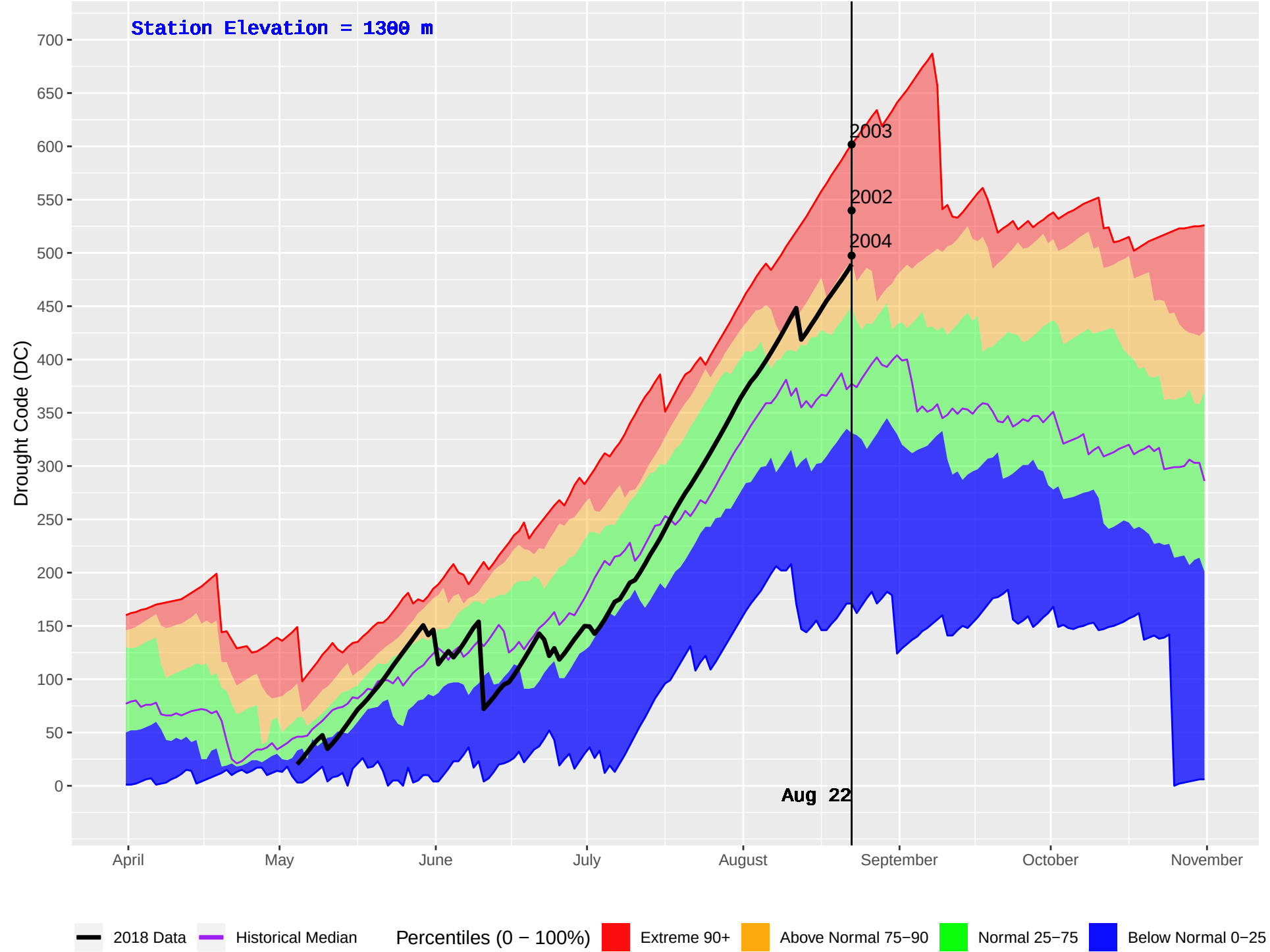
MARION (367) : Historical (1994–2016) and Current (2018) Daily Drought Code (DC)
