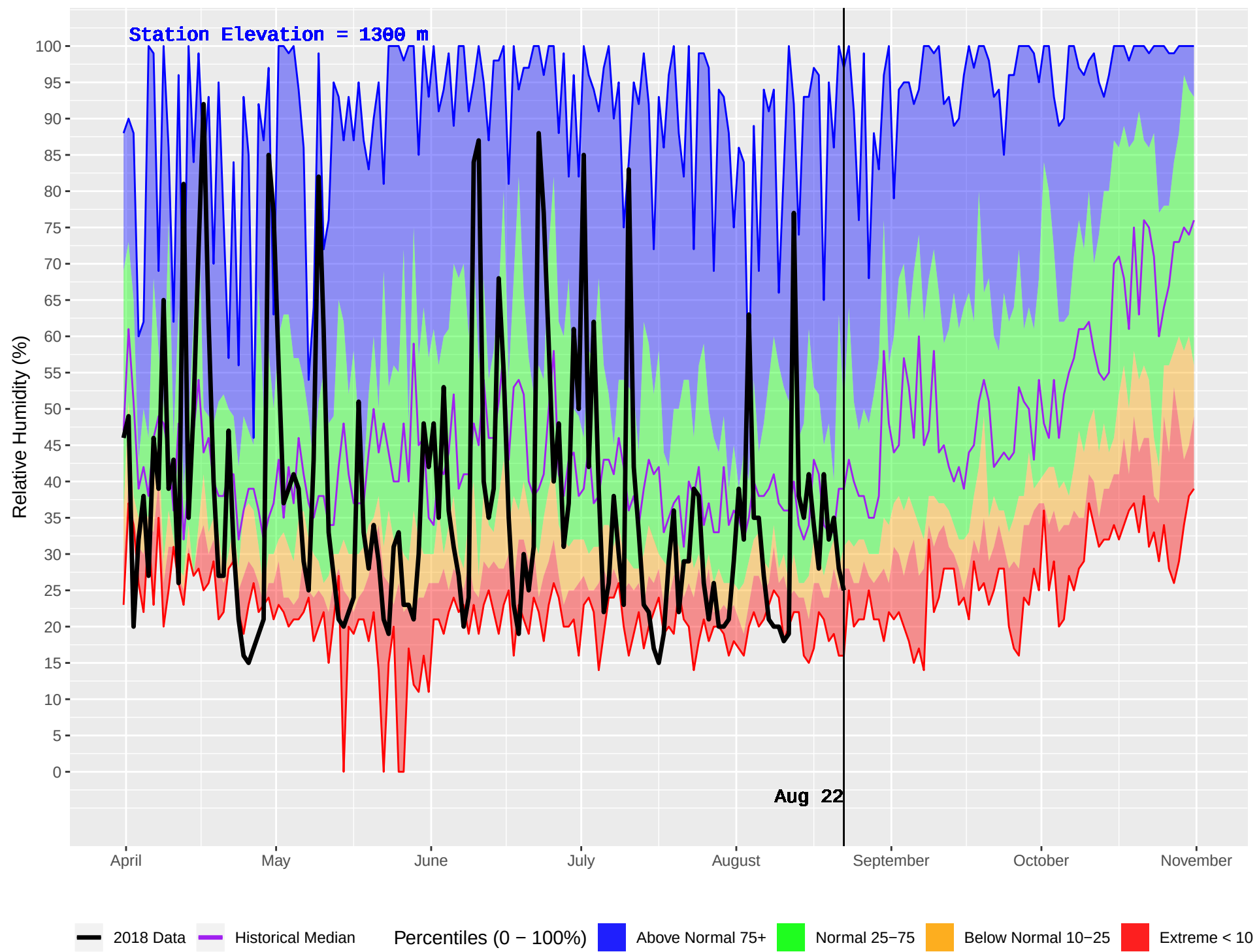
MARION (367) : Historical (1994–2016) and Current (2018) Daily Relative Humidity
