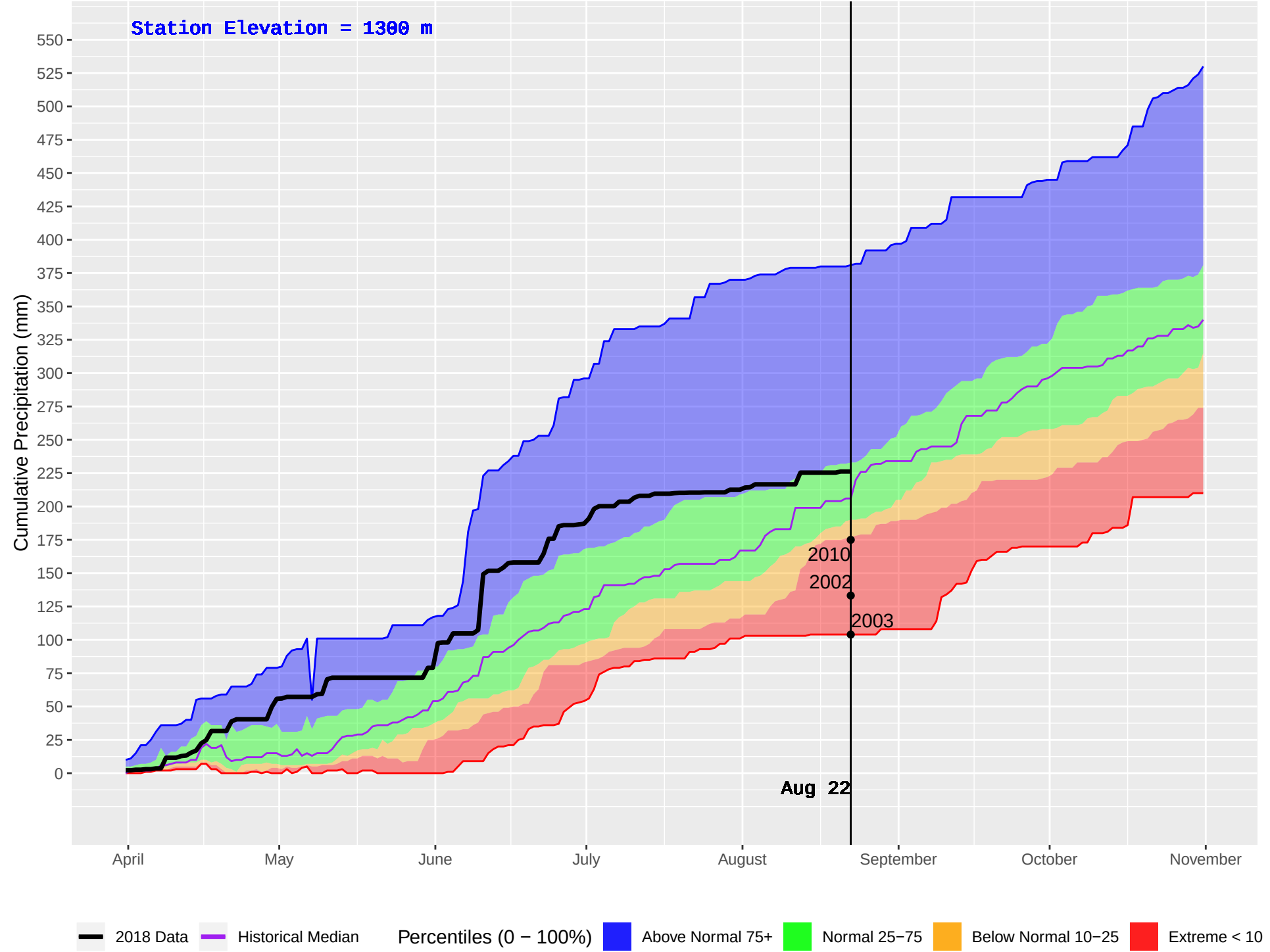
MARION (367) : Historical (1994–2016) and Current (2018) Daily Cumulative Precipitation
